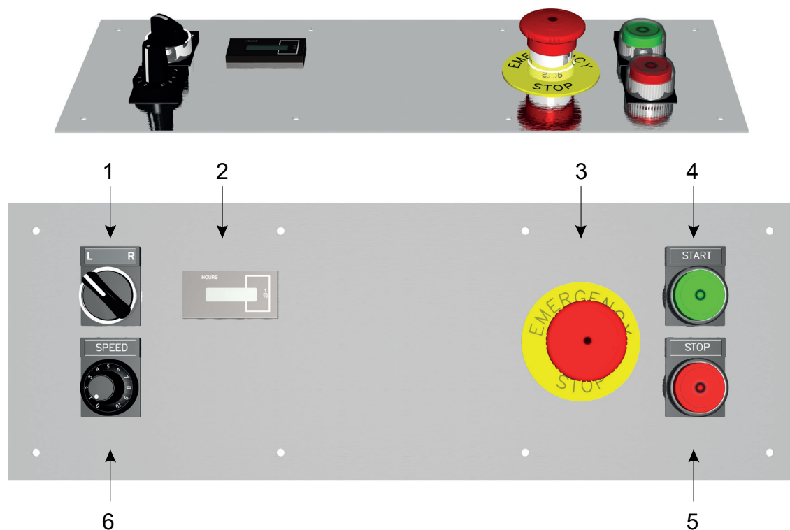
Figur 4.2 Scanmaskin 650 kontrollpanel
