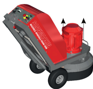
Figure 3.1 Lifting points
